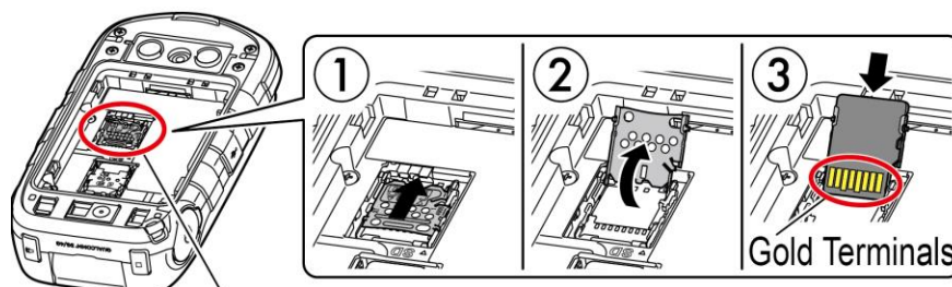
microSD Card Holder
